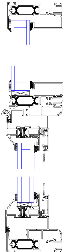
300 series shown in combination with Alwinds 480 flush glazed 3 1/2" frame.
